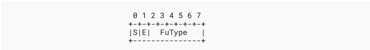
Figure 10: The Structure of FU Header
